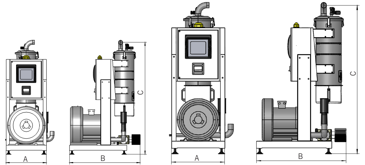
SHY-M2~M5
